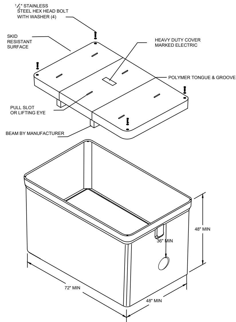
ELECTRIC PULL VAULT 6' X 4' X 4'
