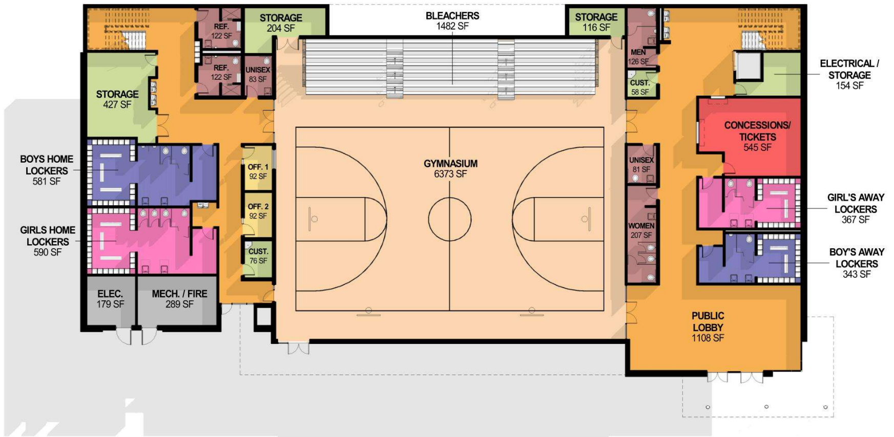
LOWER LEVEL FLOOR PLAN 17,867 GSF (29,806 TOTAL)
