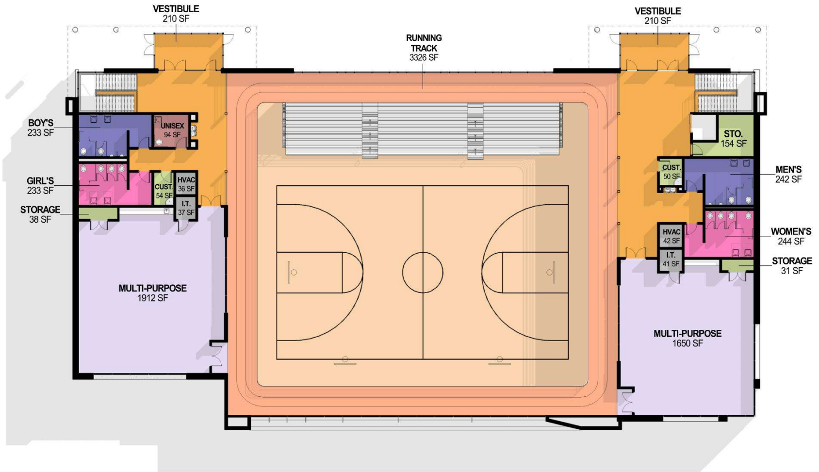
UPPER LEVEL FLOOR PLAN 11,939 GSF (29,806 TOTAL)
