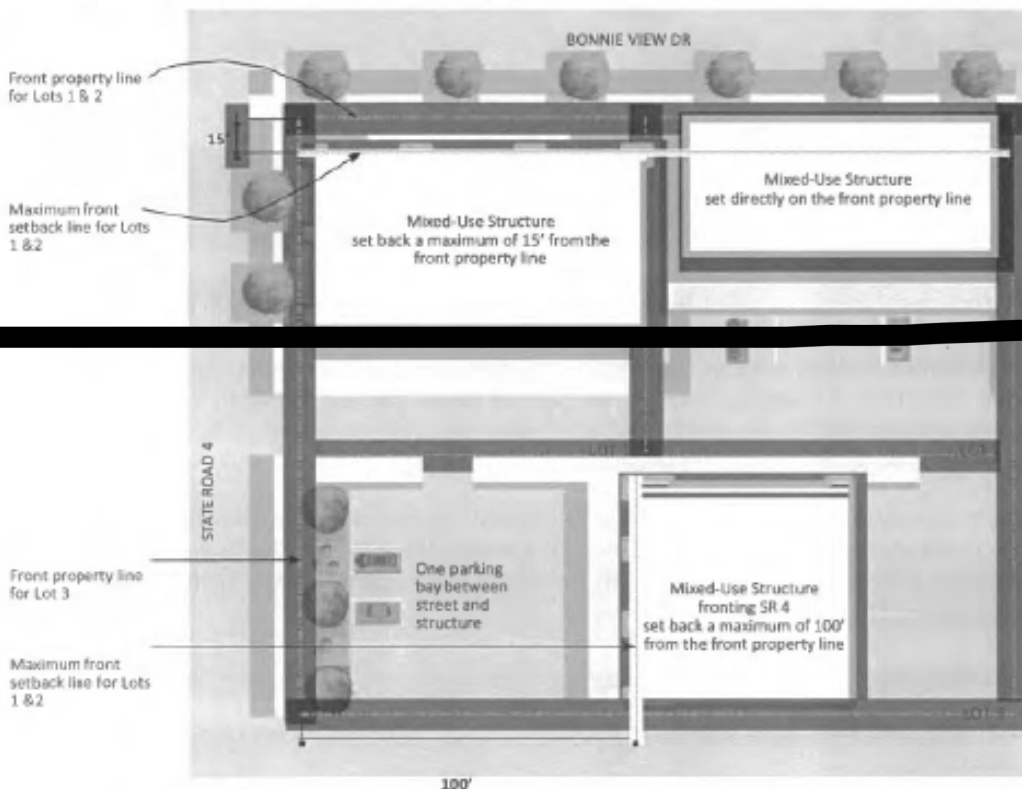
Figure 2: WRTC Site Orientation Standards
