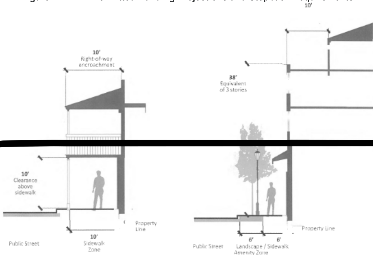
Figure 4: WRTC Permitted Building Projections and Stepback Requirements
