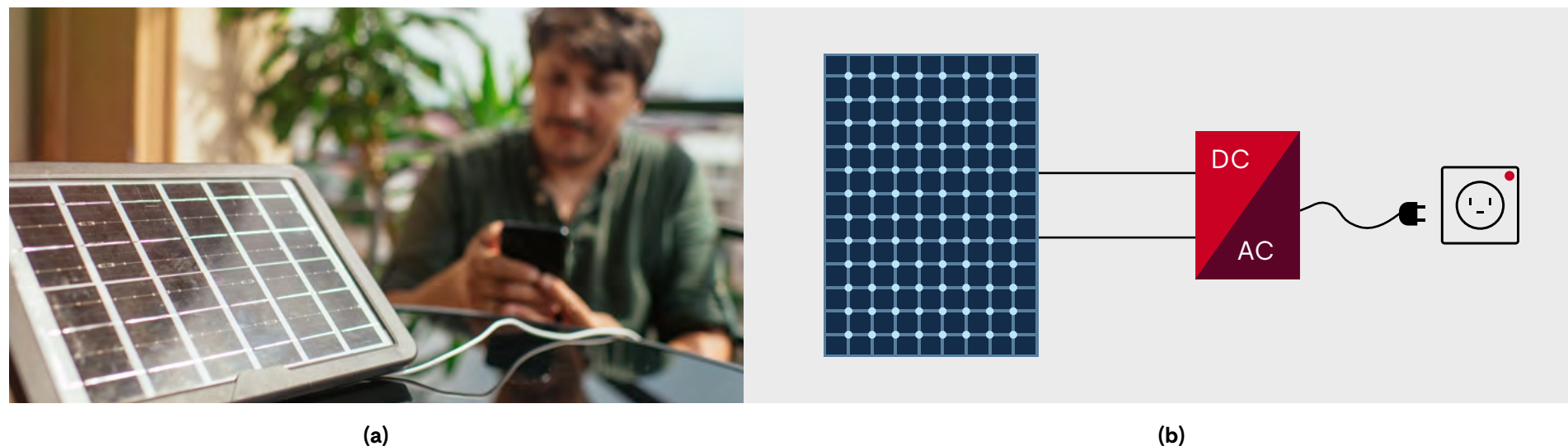
Figure 1. (a) Balcony-type PIPV module installation; (b) PIPV electrical schematic.
