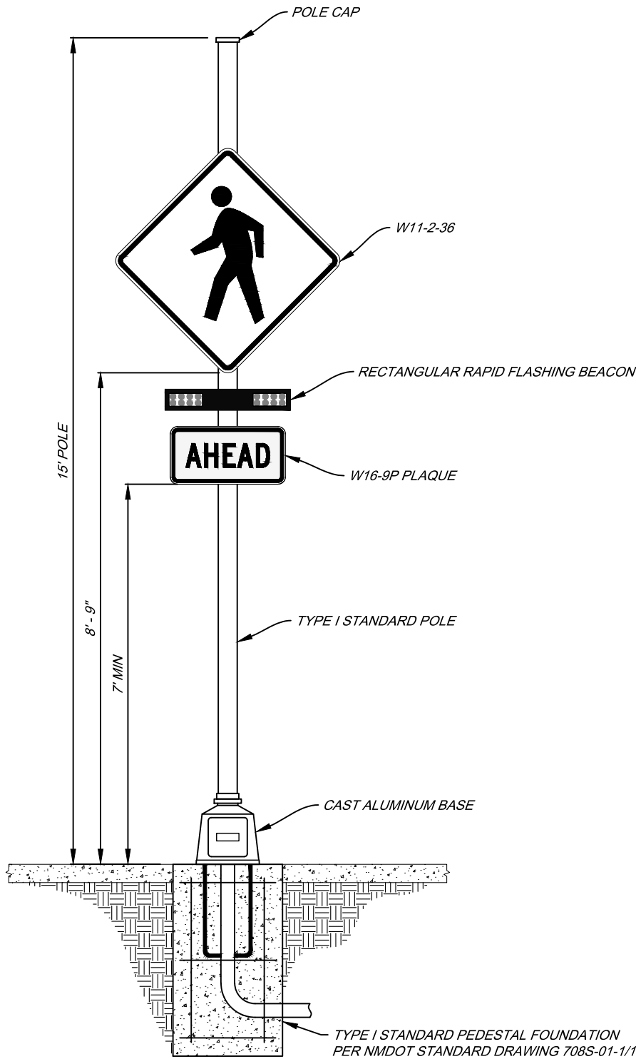
RECTANGULAR RAPID FLASHING BEACON (RRFB) TYPE I PEDESTAL POLE DETAIL A
