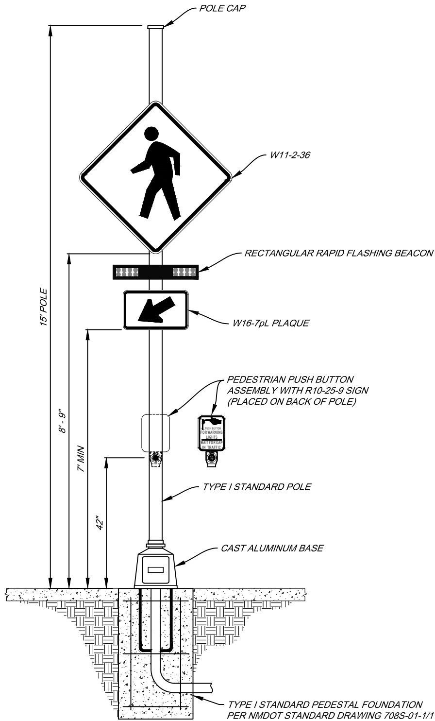
RECTANGULAR RAPID FLASHING BEACON (RRFB) TYPE I PEDESTAL POLE DETAIL B
