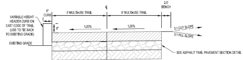
TRAIL TYPICAL SECTION LEFT SLOPING - 10' TRAIL (1%) WITH BENCH & 3:1 TIE NOT TO SCALE
